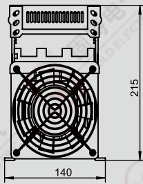
SAM3Y40300D 长宽高:345mm*140mm*215mm
