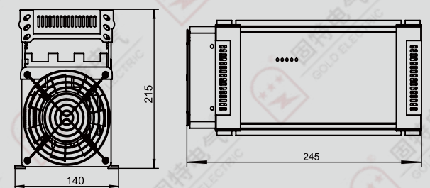
SAM3Y40200D 长宽高:245mm*140mm*215mm
