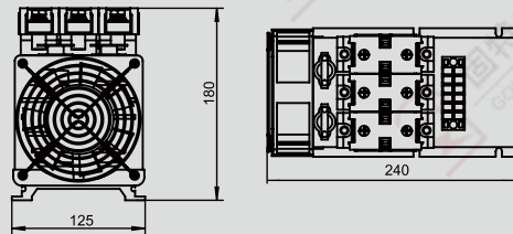
SAM3Z40150D 长宽高:240mm*125mm*180mm
