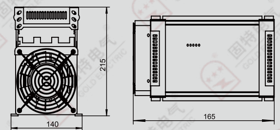
SAM3Y40120D 长宽高:145mm*140mm*215mm
